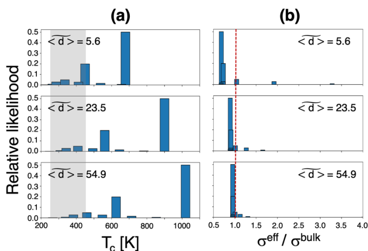
Figure 67. The computed relative likelihood for (a) the critical temperature T_c and (b) \sigma^{\text{eff}}/\sigma^{\text{bulk}} at 298 K with different LLZO grain sizes.
