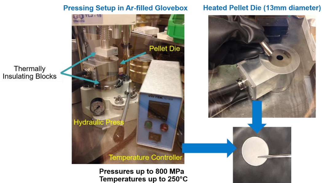
Figure 102. Hot-press setup inside an argon glove box for processing sulfide-based solid electrolyte pellets and solid-state cells.
