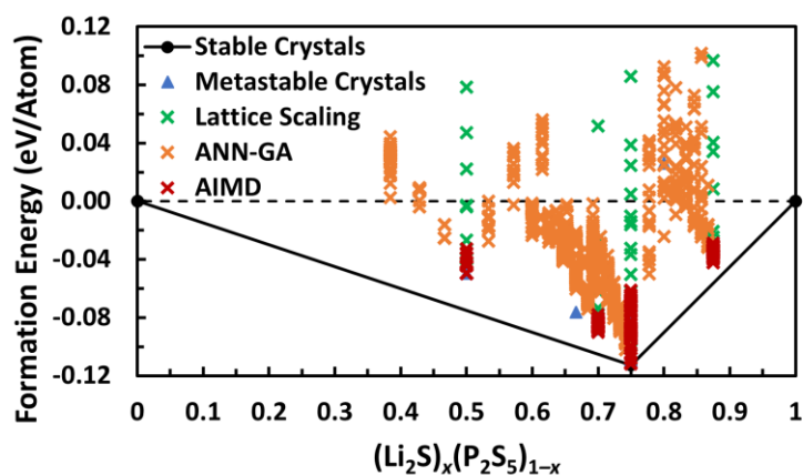
Figure 88. Phase diagram of glass/ceramic – LPS with varying compositions, including stable crystals, metastable crystals, lattice-distorted structures, amorphous phases generated either from artificial neural network – genetic algorithm or ab initio molecular dynamics simulations and recomputed with density functional theory.
