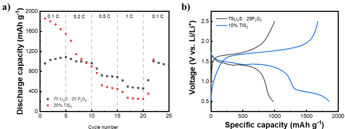
Figure 40. (a) Rate performance and (b) corresponding voltage profiles at 1 st cycle. Electrolyte used is 75Li 2 S – 25P 2 S 5 in the cathode.
