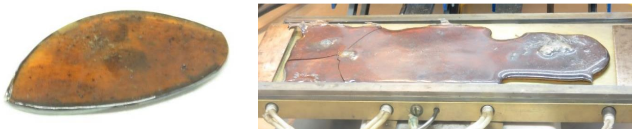
Figure 10. (a) 50 g casting of ISU-6 mixed oxy-sulfide nitride (MOSN) glassy solid electrolyte (GSE). (b) 250 g preform of ISU-6 MOSN GSE in annealing molds.
