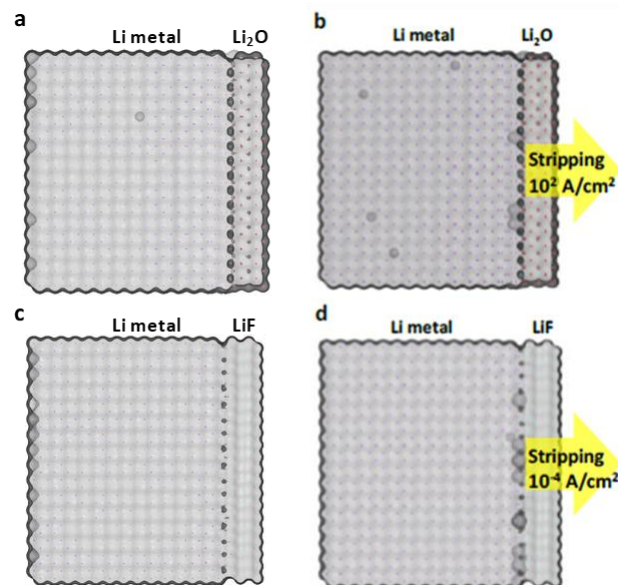
Figure 50. Kinetic Monte Carlo simulations of the stripping process. (a/c) Under stress bias ( E_p = 0.55 eV, \dot{\epsilon} = 0.01 ), the lithium surface during delithiation is smooth at both interfaces. Without the stress, (b) the lithium surface is smooth with Li 2 O layer, but (d) has trapped vacancies with LiF layer.
