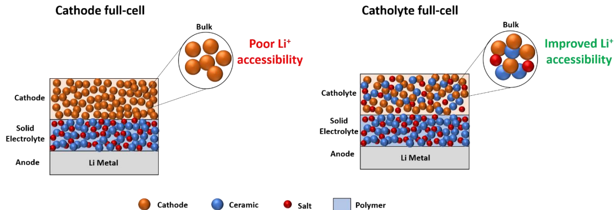
Figure 17. Schematic comparing the structures of cathode and catholyte full cells and the possible extents of their Li + accessibilities.
