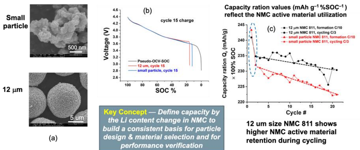
Figure 128. Electrochemical diagnostic analysis and characterization by Idaho National Laboratory to uncover utilization and degradation of cathode active material.
