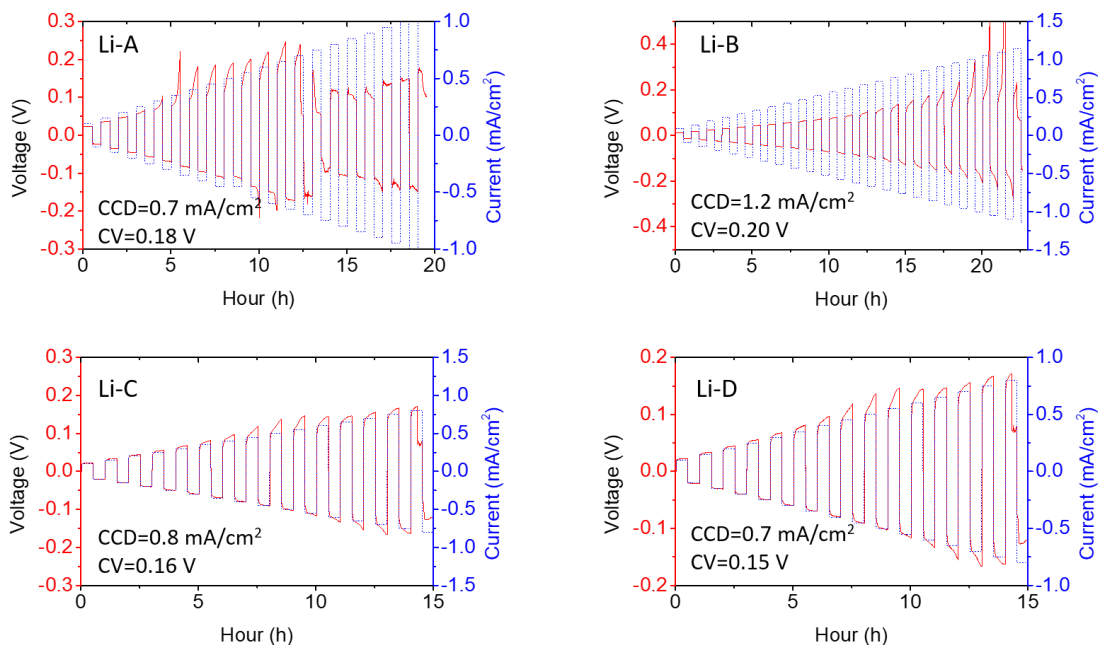
Figure 25. Lithium plating/stripping behaviors for the LiX|LLZTO|LiX cells at a step-increase current for 0.5 hours. Four cells with four different surface modifications of A, B, C, and D. The determined critical current density and critical overpotential are listed.
