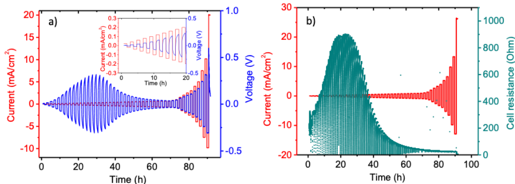
Figure 43. (a) Voltage profiles of a Li|LYC|Li symmetrical cell during the step-increase of current density and (b) corresponding cell resistance. Inset in (a) shows the voltage profile during the first 20 hours. The current density step size is 0.02 \text{ mA/cm}^2 , and the duration of each charge/discharge step is 1 hour.
