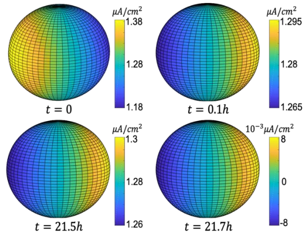
Figure 59. Current density distribution in the void.
