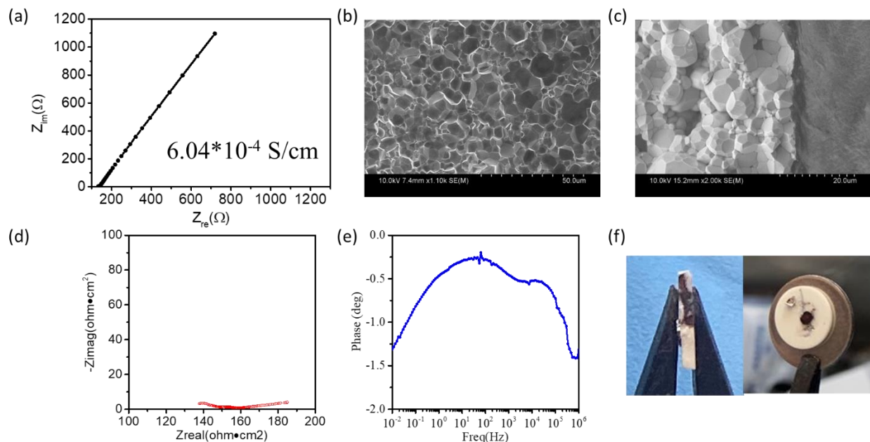
Figure 24. Electrochemical properties of LLZTO solid electrolyte pellet. (a) Electrochemical impedance spectroscopy (EIS) plot of Au|LLZTO|Au cell and calculated total ionic conductivity. (b) Particle morphologies distribution. (c) Scanning electron microscopy of Li-alloy|LLZTO interface. (d) EIS plot and (e) Bode plot for a LiC|LLZTO|LiC cell. (f) Optical picture of shorted LLZTO.
