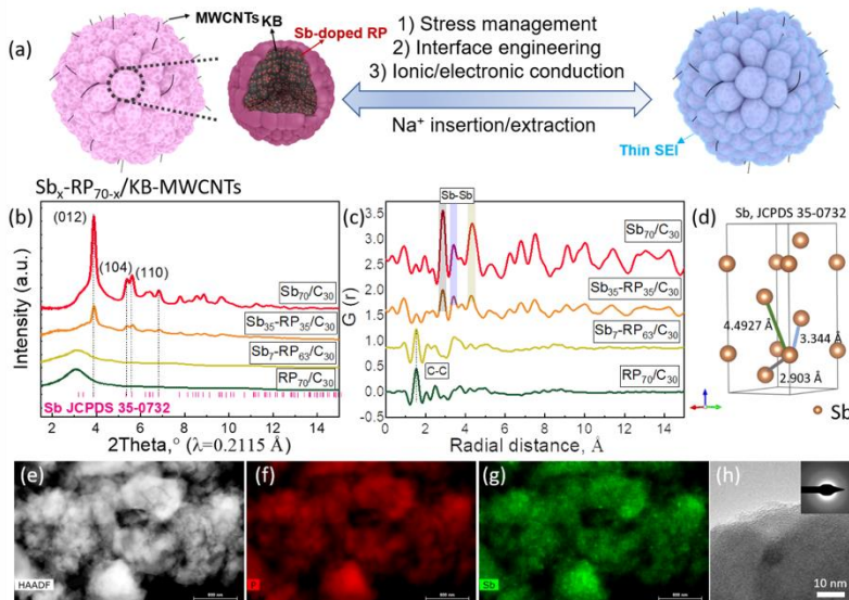
Figure 116. (a) Schematic illustration of the structure of hierarchical micro/nanostructured Sb_x-RP_{70-x}/C_{30} composite before and after cycling. (b) High-resolution X-ray diffraction and (c) pair distribution function data for Sb_x-RP_{70-x}/C_{30} composite. (d) Crystal structure of standard antimony (JCPDS 35-0732) with interatomic Sb-Sb distance index. (e) High-angle annular dark-field imaging transmission electron microscopy image. (f) Phosphorus elemental mapping. (g) Antimony elemental mapping. (h) Selected area electron diffraction pattern of Sb_7-RP_{63}/C_{30} composite.
