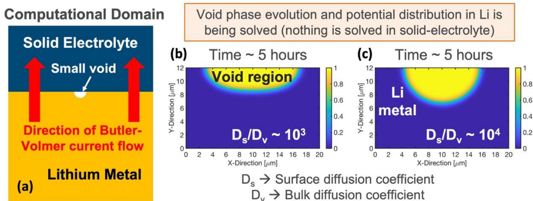
Figure 57. (a) Schematic of the computational domain where evolution of the surface void is being investigated. Flow of current and evolution of void space within lithium is studied. Nothing is being solved in the electrolyte. (b-c) Snapshot of a void after 5 hours of stripping, with ratio of surface over bulk diffusion coefficient being 10^3 and 10^4 , respectively.
