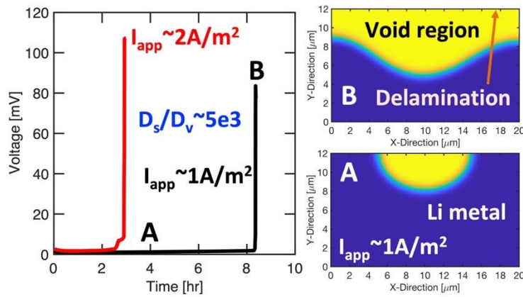
Figure 58. Voltage versus time response during the evolution of a void at the Li/electrolyte interface. Due to higher exchange current densities, the potential drop at interface is minimal. However, as the voids start to span the entire domain, the potential starts to increase rapidly. Partially and completely delaminated structures are pointed out by “A” and “B,” which are obtained after lithium stripping for 4 and 8.5 hours, respectively. Increasing current density from 1 A/m 2 to 2 A/m 2 quickens the delamination process. Also, the surface diffusion coefficient is assumed to be 5 \times 10^3 times larger than the bulk diffusivity.
