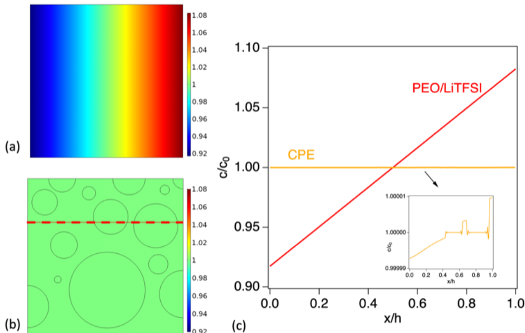
Figure 96. Lithium cation concentration maps in (a) PEO/LiTFSI binary electrolyte and (b) composite electrolyte of PEO/LiTFSI and LIGC™ particles. (c) Comparison of the two scenarios along the cross-section (b, red line). Normalized concentrations and distances are shown. Significant reduction in gradients can be seen with addition of LIGC™. When plotted on a separate scale, the \text{Li}^+ concentration shows some variation (c, inset); cross-sections of the two LIGC™ particles can be clearly identified where the concentration remains constant.
