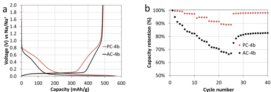
Figure 120. (a) 1 st cycle voltage profile and (b) rate performance of PC-4b and AC-4b in sodium half-cell (90 wt% AM: 5 wt% SP: 5 wt% PAA) performed in a potential range of 5 mV - 2 V with 1 M NaPF 6 in EC/DMC (1:1 in weight) as electrolyte.
