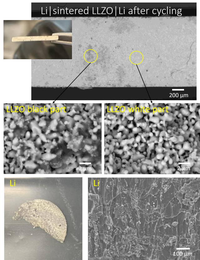
Figure 93. Postmortem analysis of Li|sintered LLZO|Li. (Top row) Cross-sectional scanning electron microscopy (SEM) image of the sintered LLZO pellet after cycling. Inset: digital photograph of pellet. (Middle row) Zoomed-in SEM images of the LLZO pellet, showing two distinct regions. (Bottom row) Digital photograph of lithium and SEM image of the surface of lithium that was in contact with the LLZO pellet.
